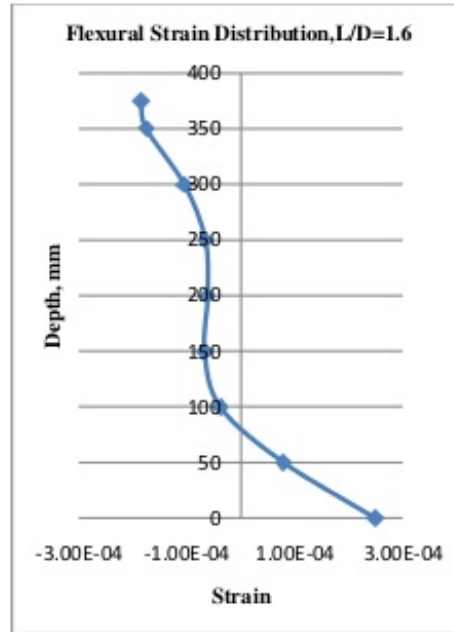
Figure 6.b. Flexural strain distribution for L/D = 1.6
