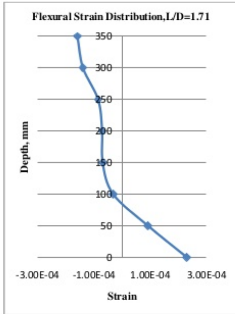
Figure 6.a. Flexural strain distribution for L/D = 1.71
