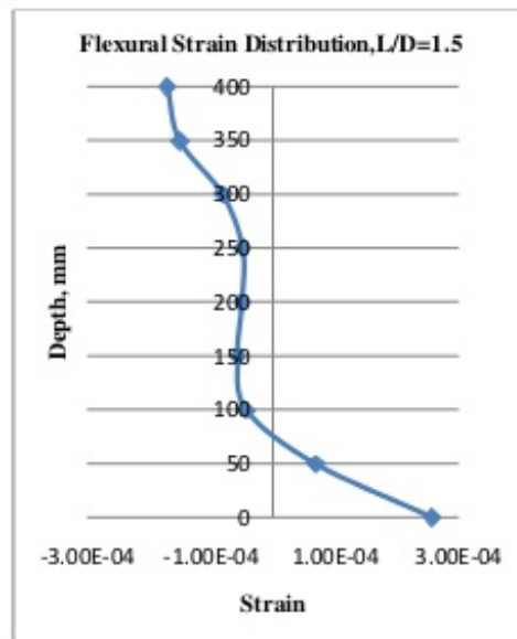
Figure 6.c. Flexural strain distribution for L/D = 1.5
